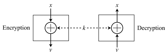
Figure 5.9 Invertibility of the exclusive-or operation
