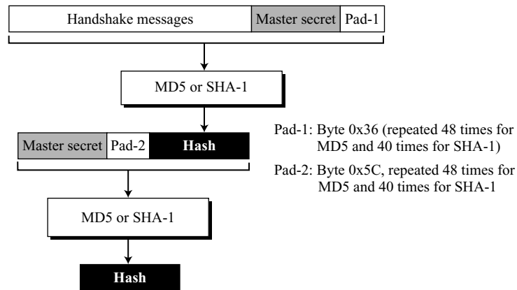
Figure 17.35 Hash calculation for CertificateVerify message
