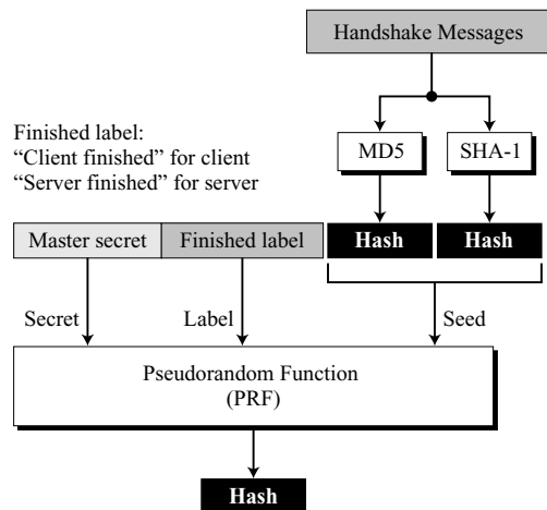
Figure 17.45 Hash for Finished message in TLS
