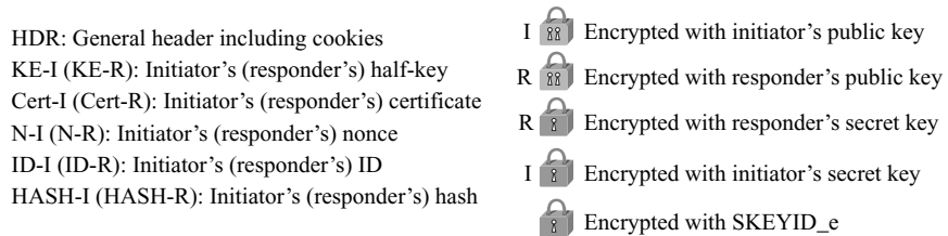
Figure 18.26 Aggressive mode, revised public-key method
