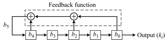
Figure 5.24 LFSR for Example 5.18
