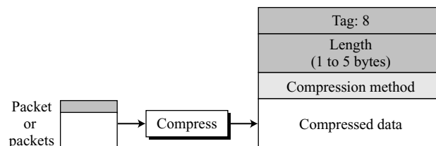
Figure 16.14 Compressed data packet
