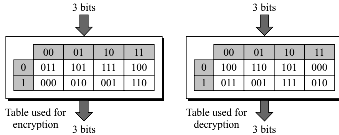
Figure 5.8 S-box tables for Example 5.11
