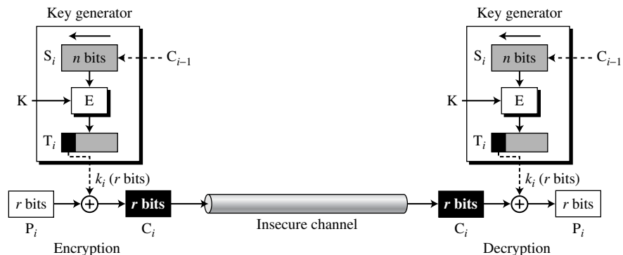
Figure 8.5 Cipher feedback (CFB) mode as a stream cipher
