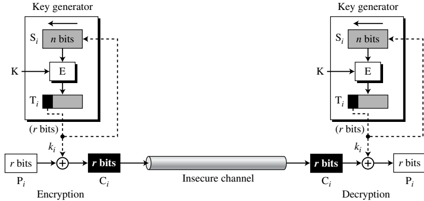
Figure 8.7 Output feedback (OFB) mode as a stream cipher
