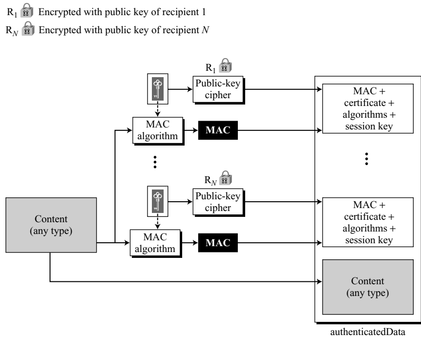
Figure 16.30 Authenticated-data content type
