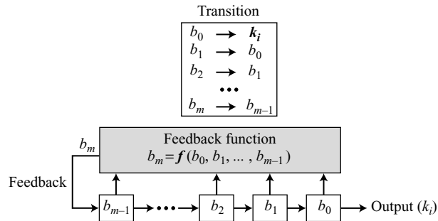
Figure 5.23 Feedback shift register (FSR)
