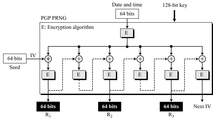
Figure K.5 PGP pseudorandom number generator
