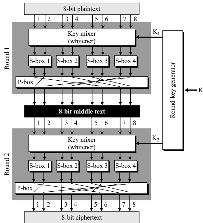
Figure 5.13 A product cipher made of two rounds
