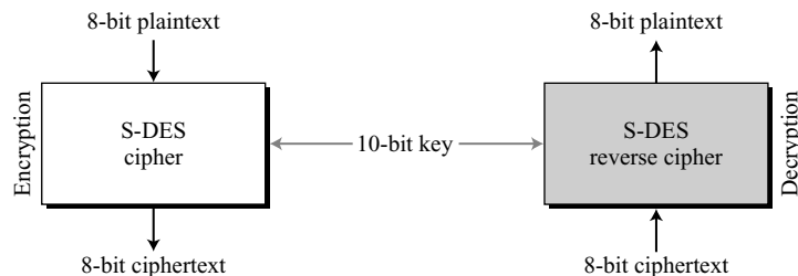
Figure O.1 Encryption and decryption with S-DES
