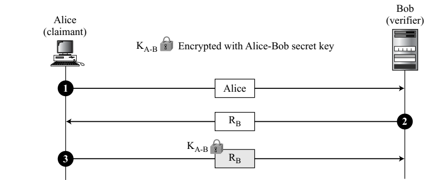
Figure 14.5 Nonce challenge
