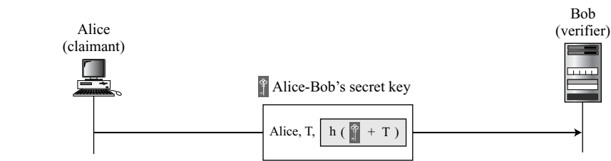
Figure 14.8 Keyed-hash function
