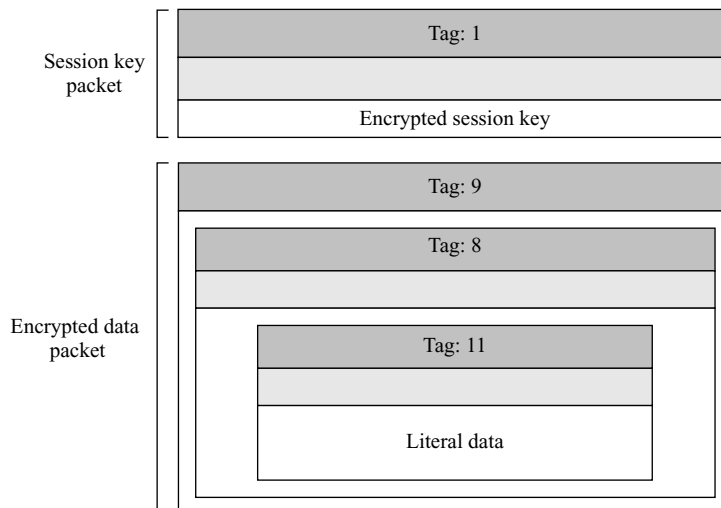
Figure 16.20 Encrypted message
