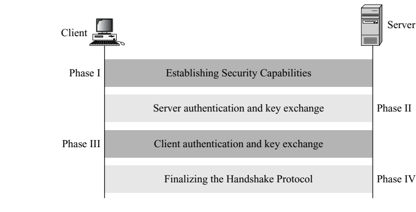
Figure 17.13 Handshake Protocol
