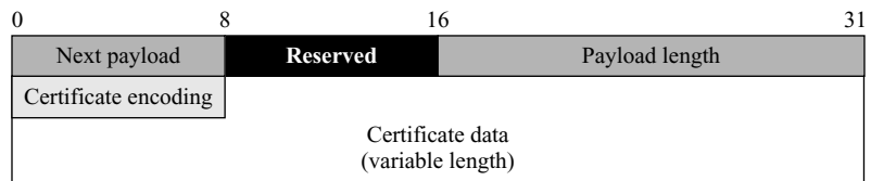
Figure 18.36 Certification payload
