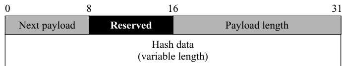
Figure 18.38 Hash payload
