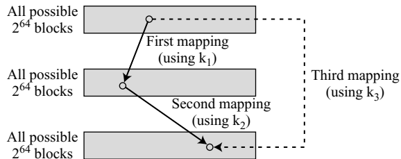
Figure 6.13 Composition of mapping
