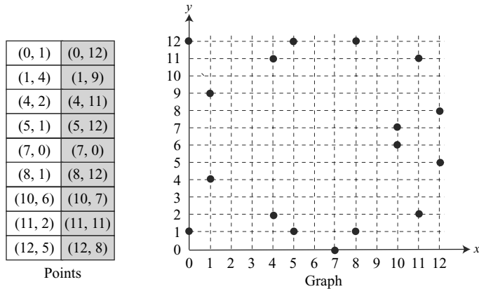
Figure 10.14 Points on an elliptic curve over GF(p)
