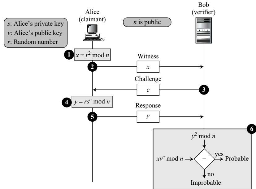
Figure 14.13 Fiat-Shamir protocol
