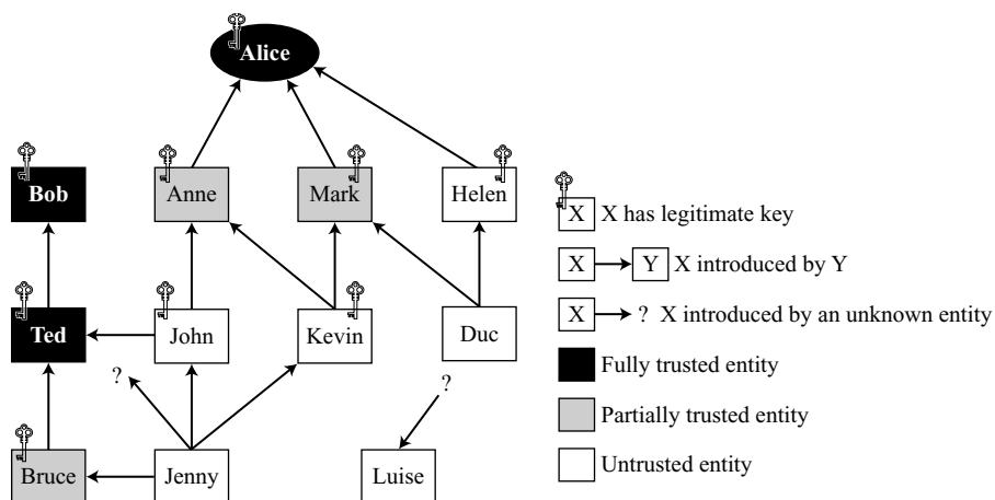
Figure 16.9 Trust model
