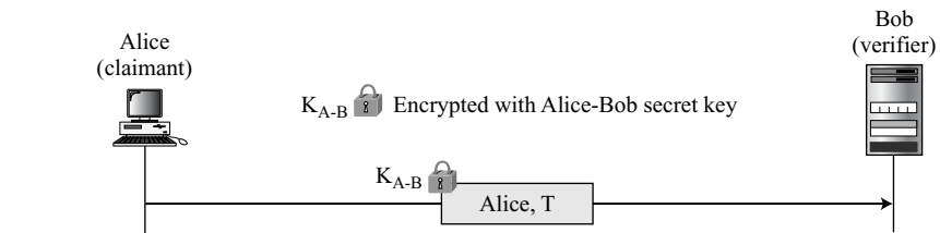
Figure 14.6 Timestamp challenge
