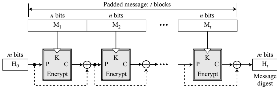
Figure 12.3 Davies-Meyer scheme
