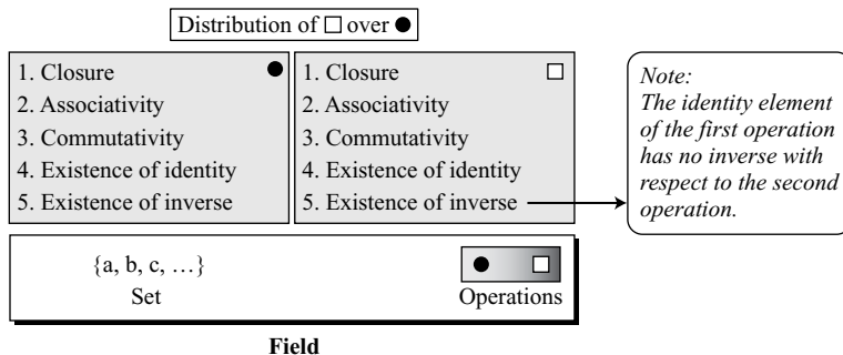
Figure 4.5 Field
