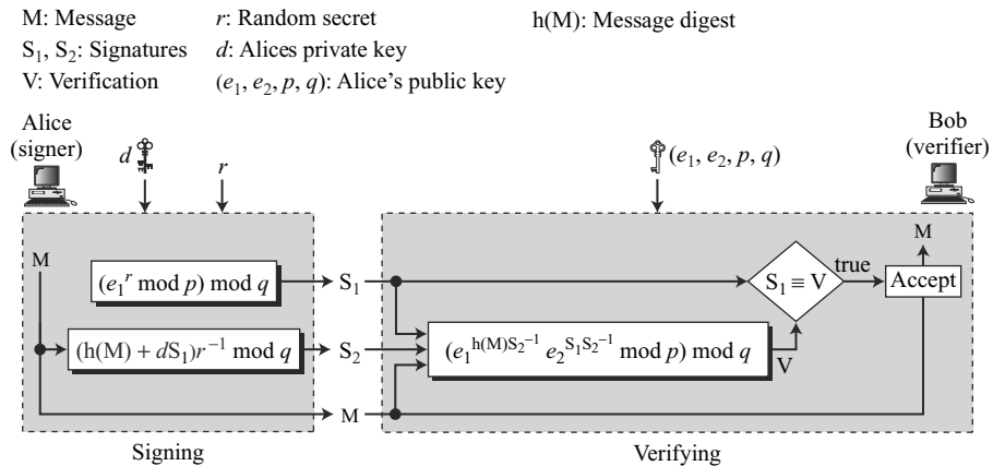
Figure 13.14 DSS scheme
