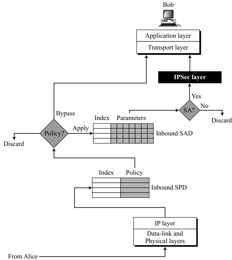
Figure 18.14 Inbound processing
