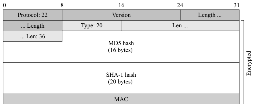
Figure 17.37 Finished message
