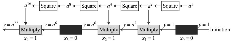
Figure 9.7 Demonstration of calculation of a^{22} using square-and-multiply method
