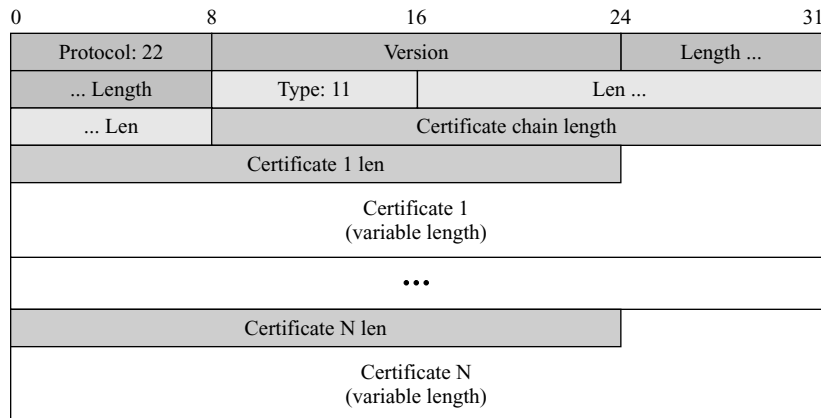
Figure 17.30 Certificate message
