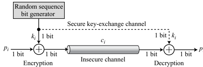
Figure 5.22 One-time pad
