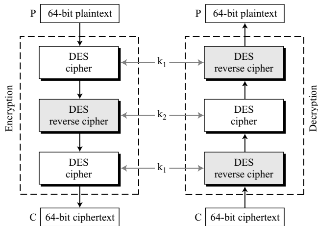
Figure 6.16 Triple DES with two keys
