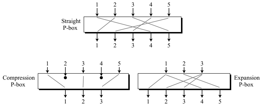
Figure 5.4 Three types of P-boxes
