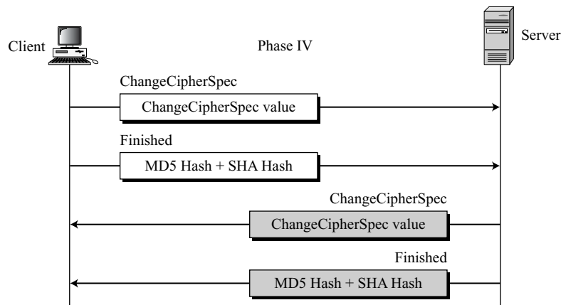
Figure 17.19 Phase IV of Handshake Protocol
