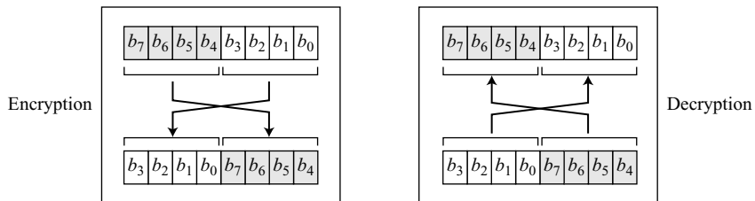
Figure 5.11 Swap operation on an 8-bit word
