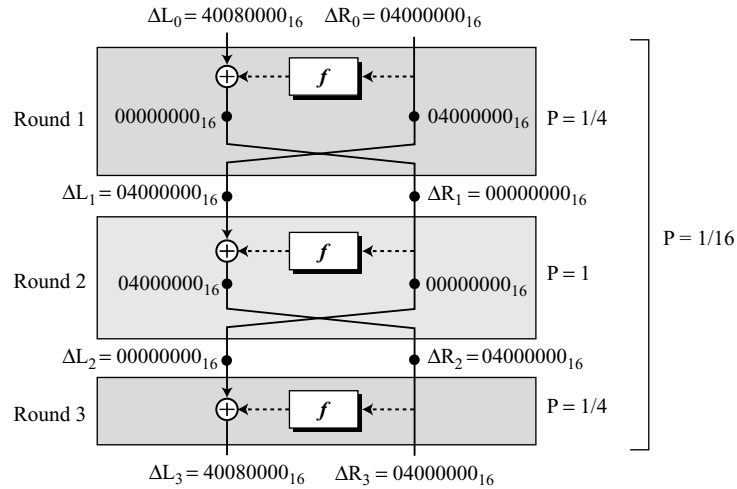
Figure N.3 A three-round characteristic for differential cryptanalysis
