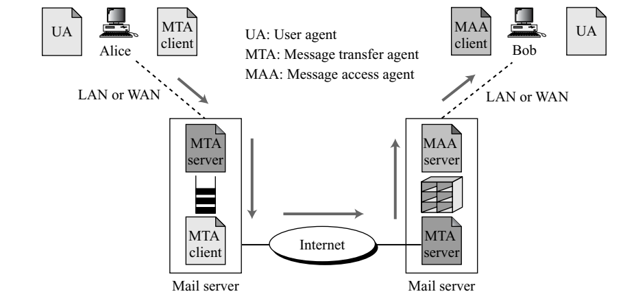
Figure 16.1 E-mail architecture
