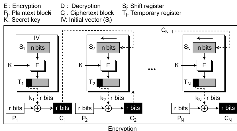
Figure 8.4 Encryption in cipher feedback (CFB) mode
