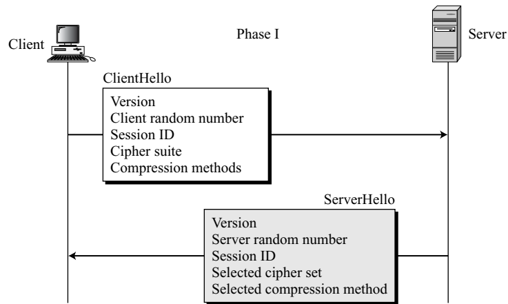
Figure 17.14 Phase I of Handshake Protocol
