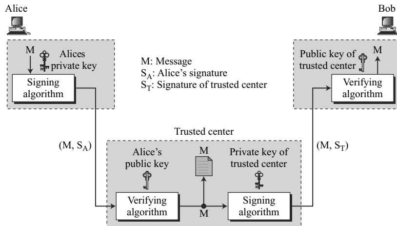
Figure 13.4 Using a trusted center for nonrepudiation
