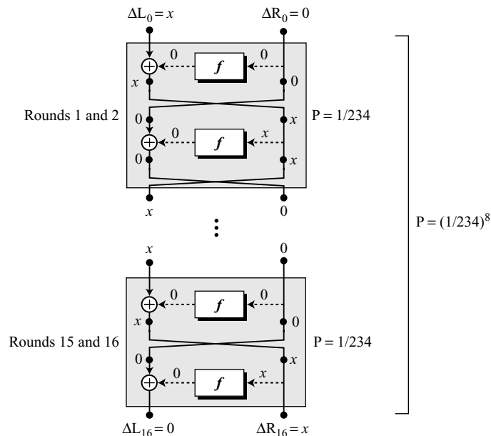
Figure N.4 A sixteen-round characteristic for differential cryptanalysis
