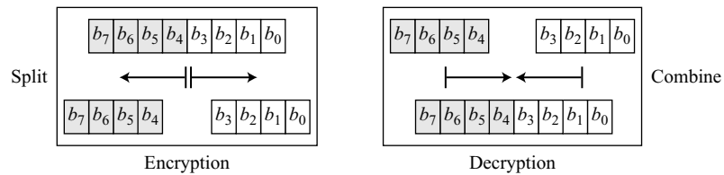
Figure 5.12 Split and combine operations on an 8-bit word
