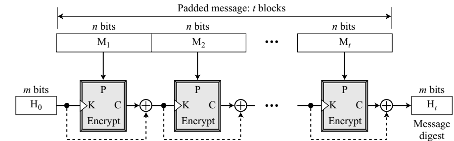
Figure 12.4 Matyas-Meyer-Oseas scheme
