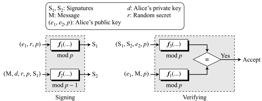
Figure 13.9 General idea behind the ElGamal digital signature scheme
