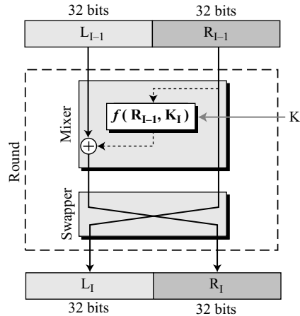
Figure 6.4 A round in DES (encryption site)
