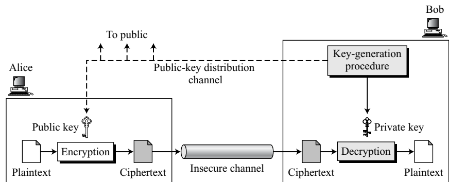
Figure 10.2 General idea of asymmetric-key cryptosystem
