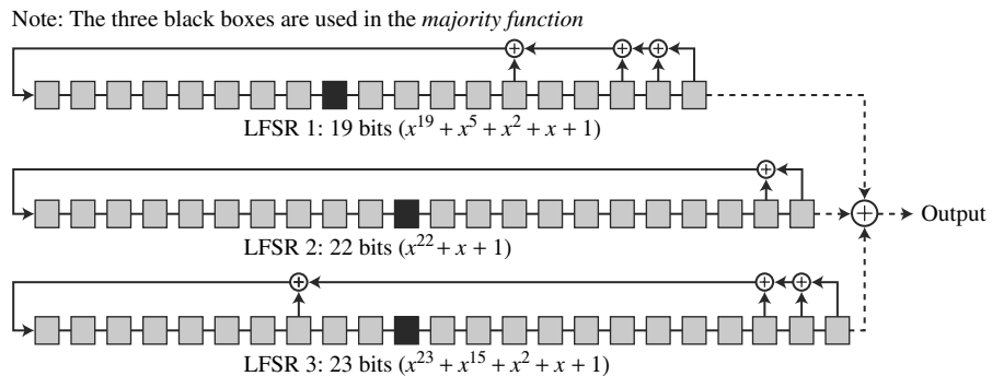
Figure 8.12 Three LFSR's in A5/1
