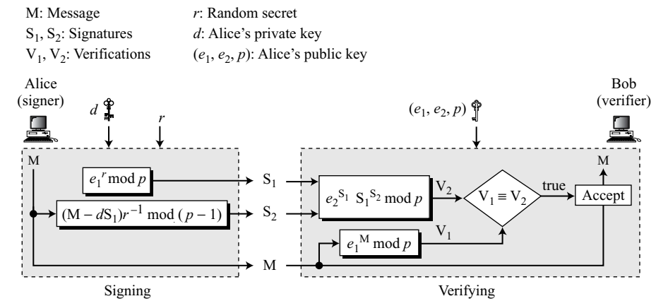
Figure 13.10 ElGamal digital signature scheme
