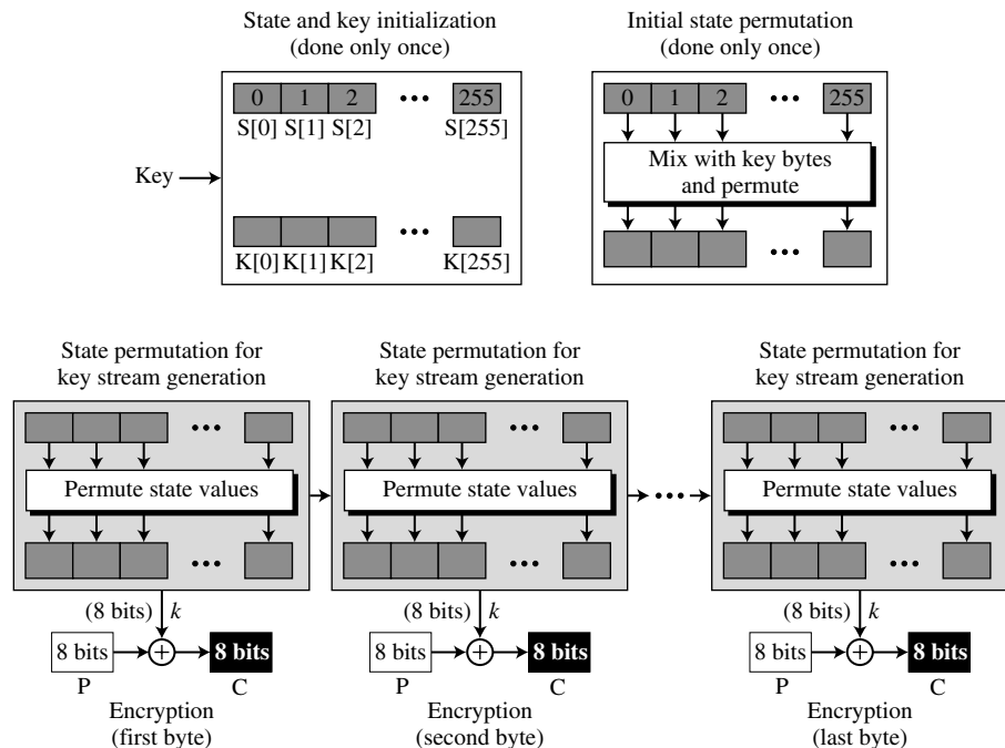
Figure 8.10 The idea of RC4 stream cipher
