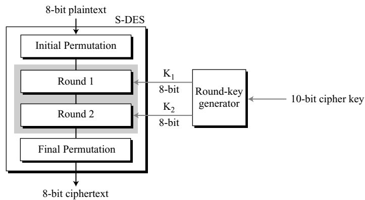
Figure O.2 General structure of S-DES encryption cipher
