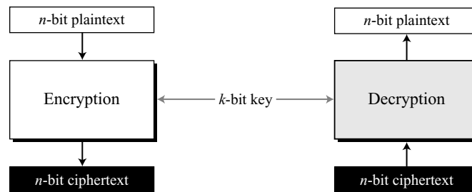
Figure 5.1 A modern block cipher
