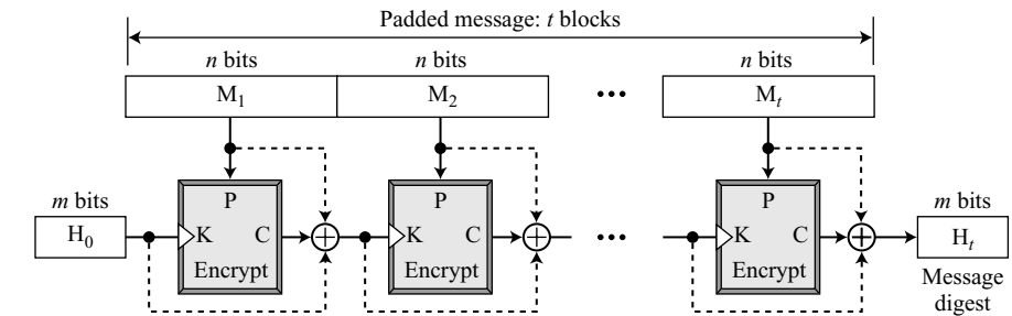
Figure 12.5 Miyaguchi-Preneel scheme
