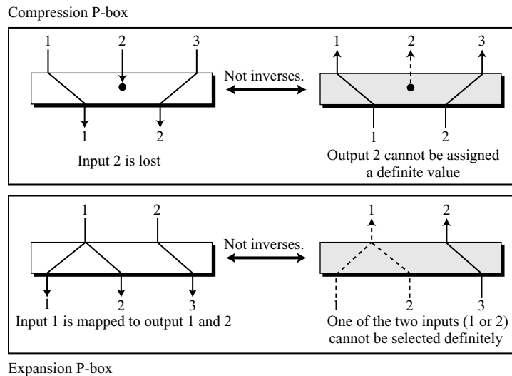
Figure 5.7 Compression and expansion P-boxes as non-invertible components
