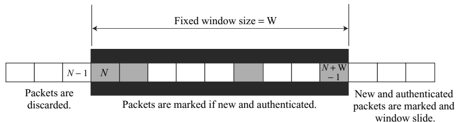
Figure 18.9 Replay window
