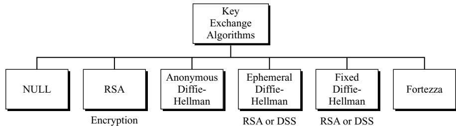
Figure 17.2 Key-exchange methods
