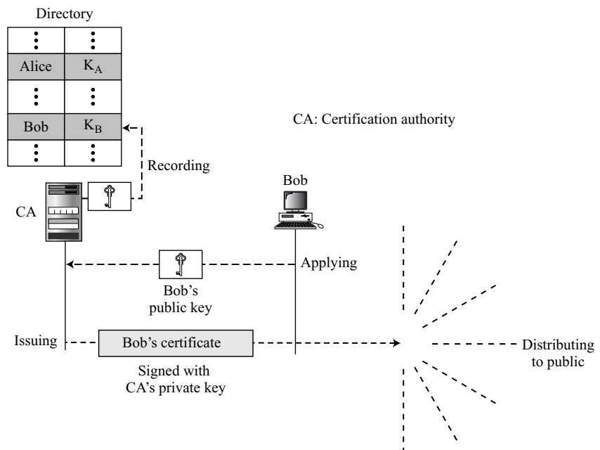
Figure 15.16 Certification authority
