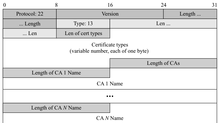
Figure 17.32 CertificateRequest message
