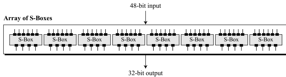
Figure 6.7 S-boxes
