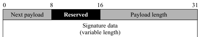
Figure 18.39 Signature payload
