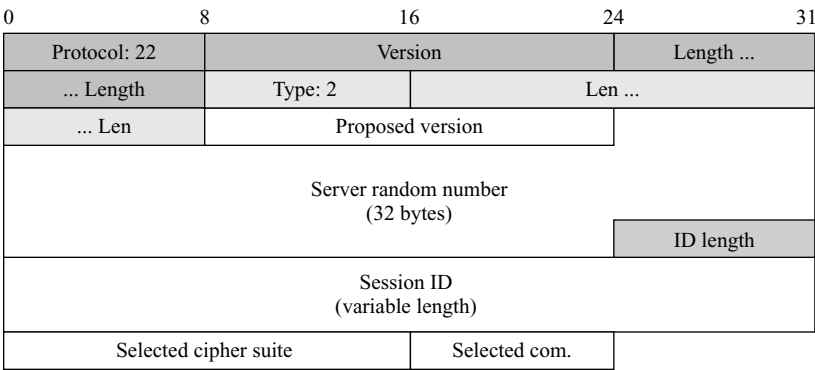
Figure 17.29 ServerHello message
