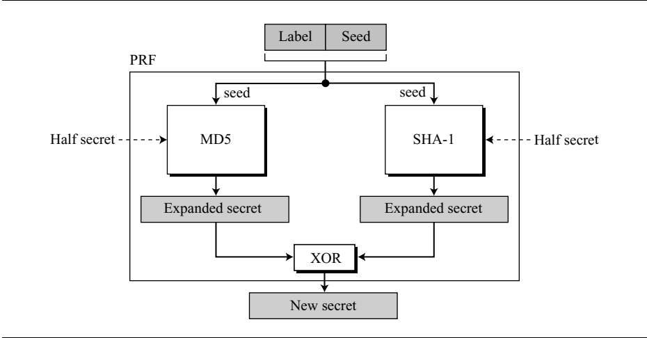
Figure 17.41 PRF
