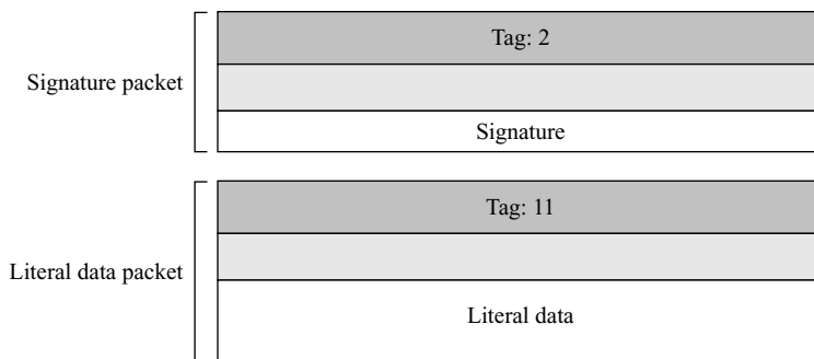
Figure 16.21 Signed message
