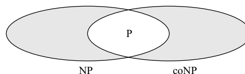
Figure L.1 Classes P, NP, and coNP
