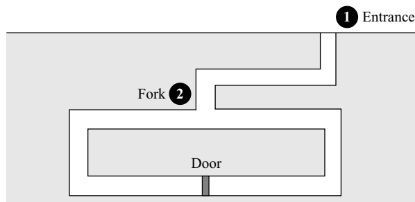
Figure 14.14 Cave example
