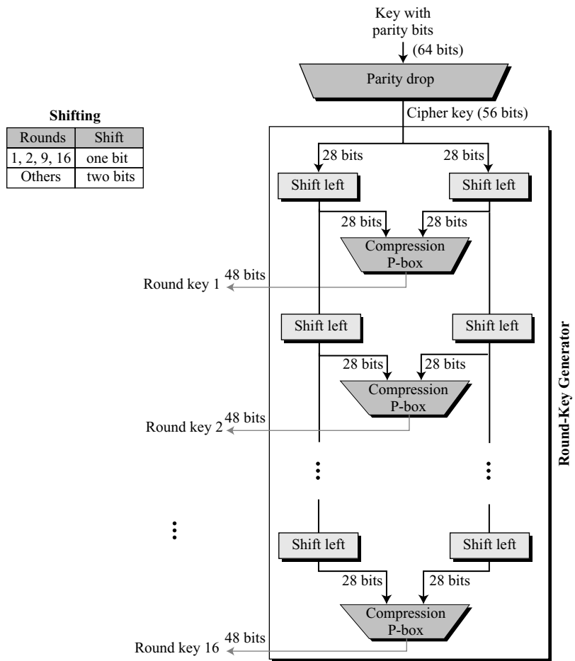
Figure 6.10 Key generation
