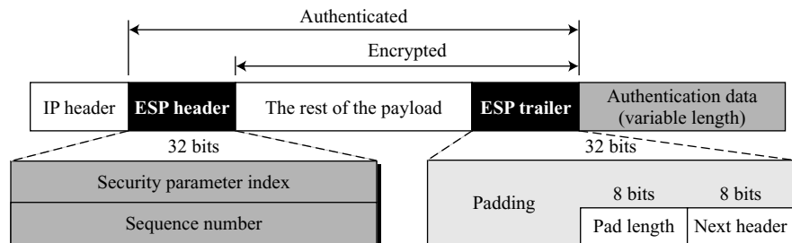
Figure 18.8 ESP
