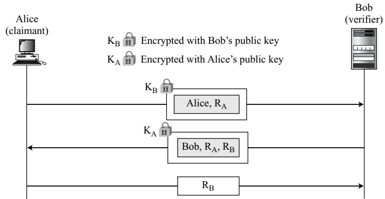
Figure 14.10 Bidirectional, asymmetric-key
