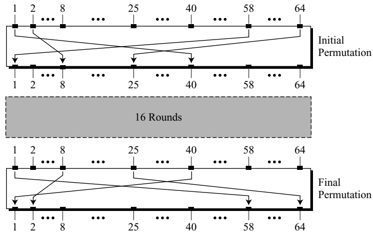
Figure 6.3 Initial and final permutation steps in DES
