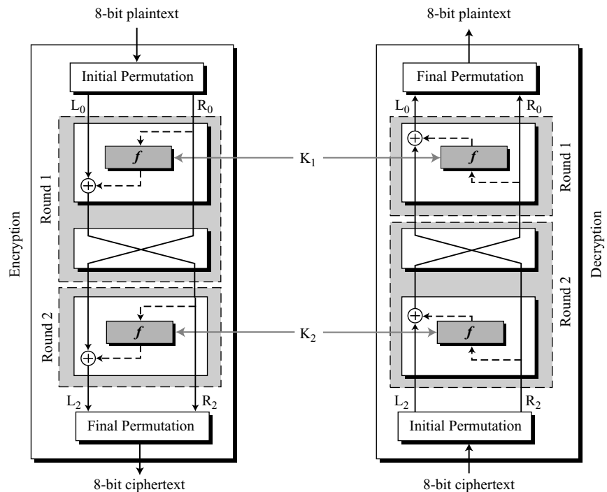
Figure O.9 S-DES cipher and reverse cipher
