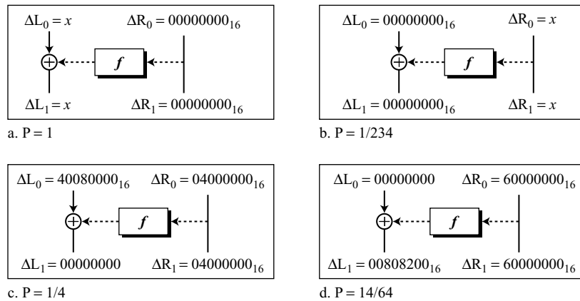
Figure N.2 Some round characteristics for differential cryptanalysis
