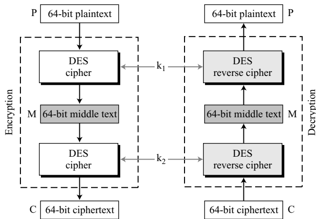
Figure 6.14 Meet-in-the-middle attack for double DES
