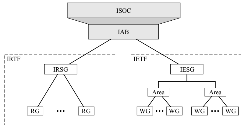
Figure B.3 Internet administration
