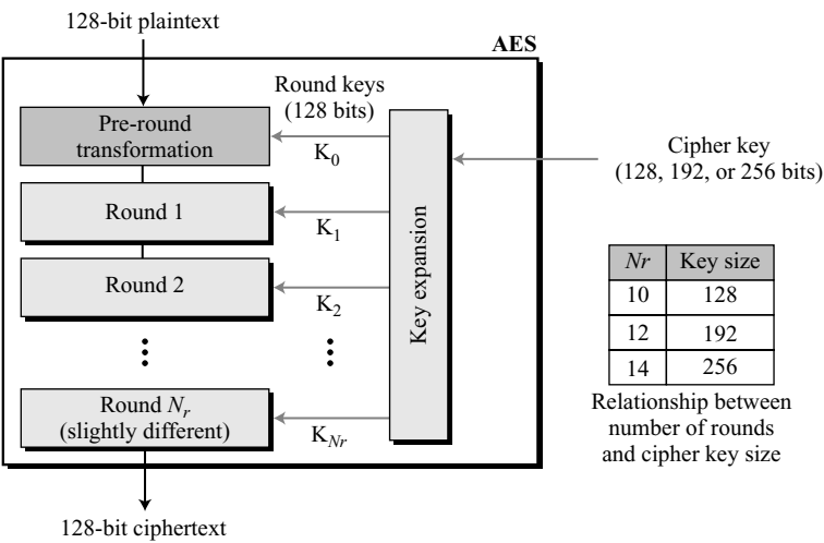
Figure 7.1 General design of AES encryption cipher
