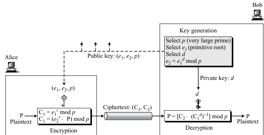
Figure 10.11 Key generation, encryption, and decryption in ElGamal
