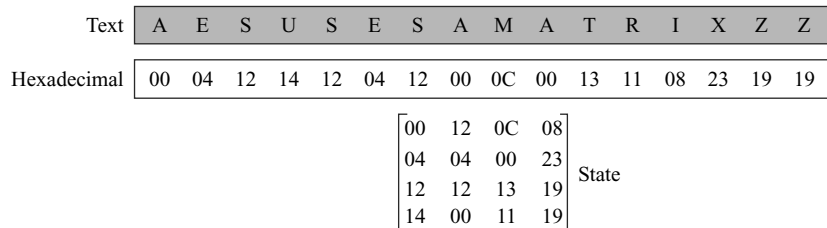
Figure 7.4 Changing plaintext to state
