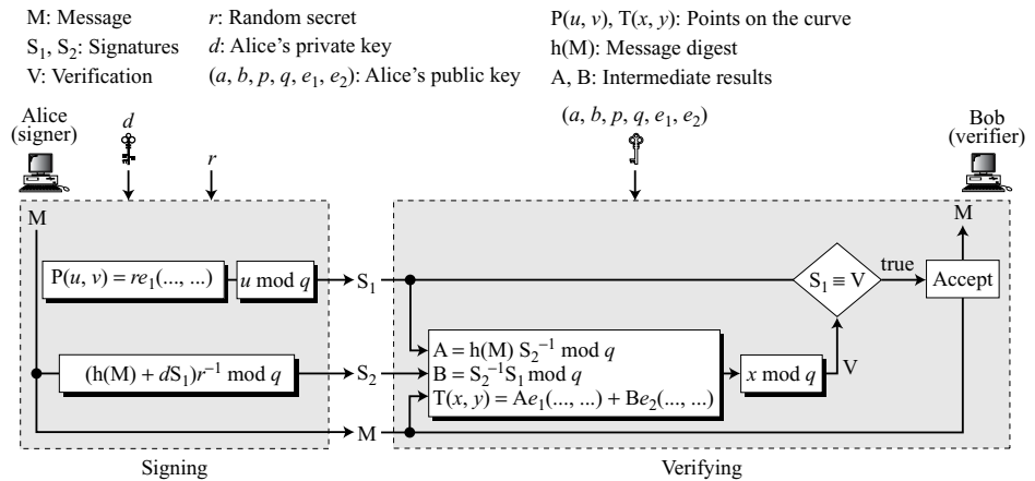
Figure 13.16 The ECDSS scheme
