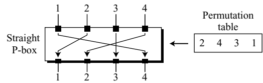
Figure O.7 Straight P-Box
