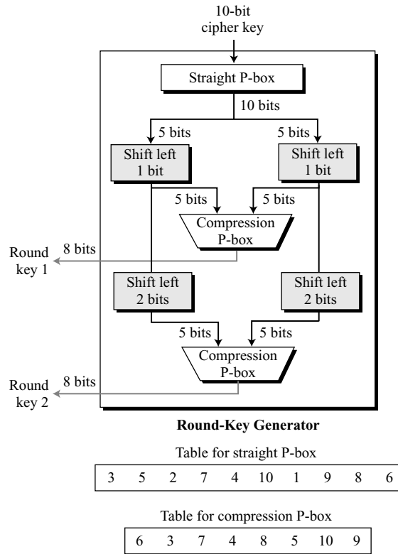
Figure O.8 Key generation
