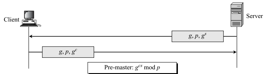
Figure 17.4 Anonymous Diffie-Hellman key exchange
