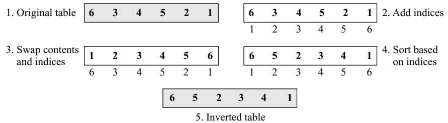
Figure 5.6 Inverting a permutation table
