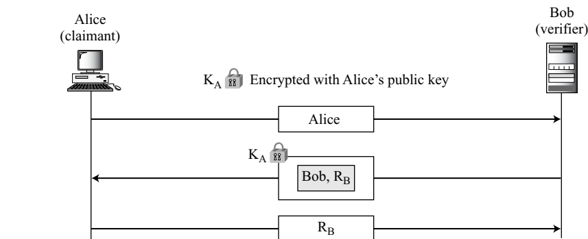
Figure 14.9 Unidirectional, asymmetric-key authentication
