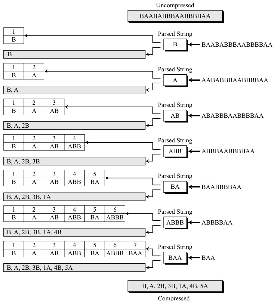
Figure M.1 Example of LZ77 encoding
