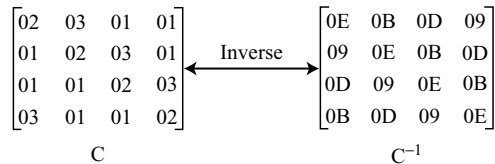
Figure 7.12 Constant matrices used by MixColumns and InvMixColumns
