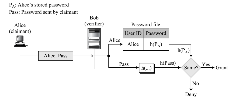
Figure 14.2 Hashing the password
