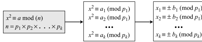
Figure 9.5 Decomposition of congruence modulo a composite
