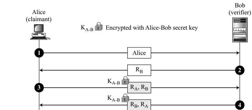
Figure 14.7 Bidirectional authentication
