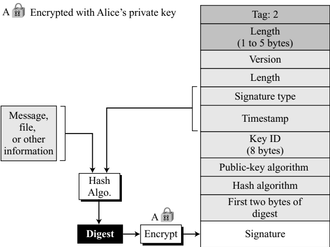
Figure 16.16 Signature packet
