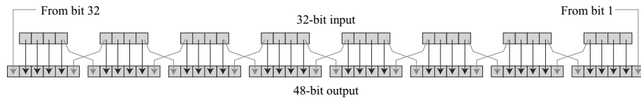
Figure 6.6 Expansion permutation
