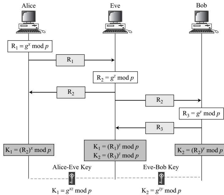
Figure 15.11 Man-in-the-middle attack
