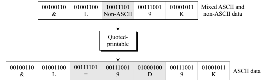
Figure 16.26 Quoted-printable
