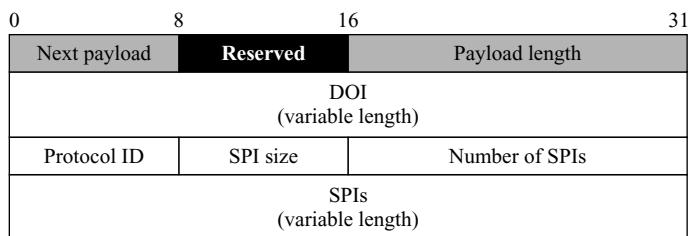
Figure 18.42 Delete payload
