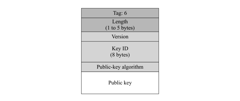
Figure 16.18 Public-key packet
