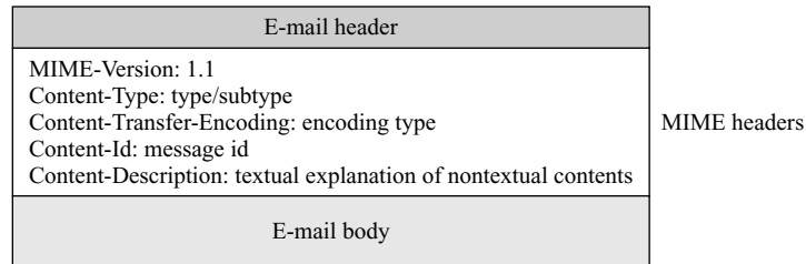
Figure 16.24 MIME header
