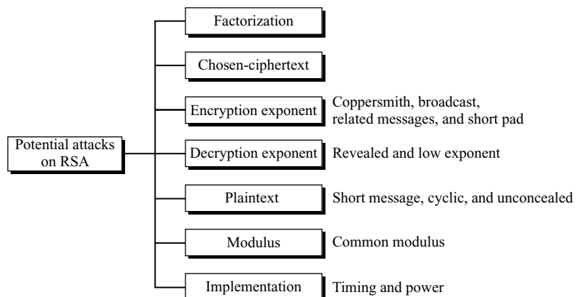
Figure 10.8 Taxonomy of potential attacks on RSA
