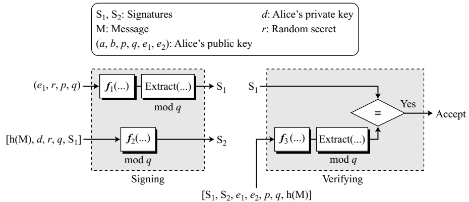
Figure 13.15 General idea behind the ECDSS scheme
