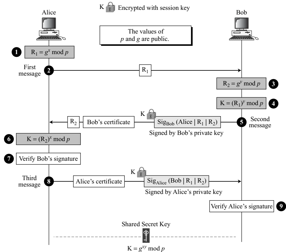
Figure 15.12 Station-to-station key agreement method
