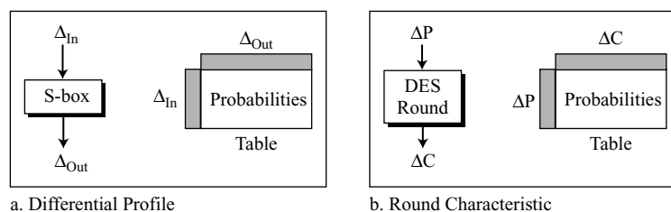
Figure N.1 Differential profile and round characteristic for DES
