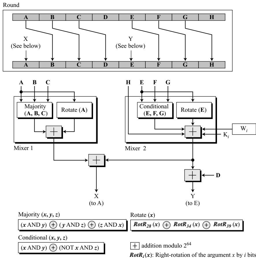
Figure 12.11 Structure of each round in SHA-512
