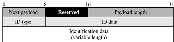
Figure 18.35 Identification payload
