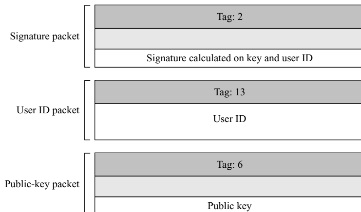
Figure 16.22 Certificate message
