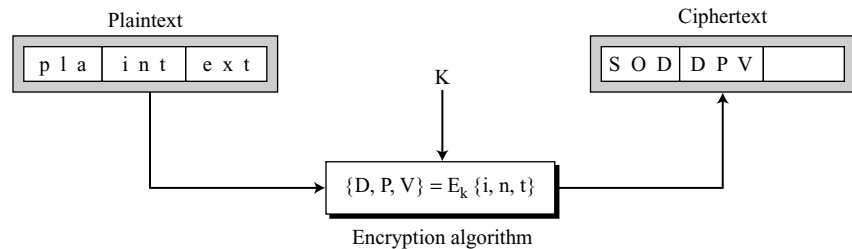
Figure 3.27 Block cipher
