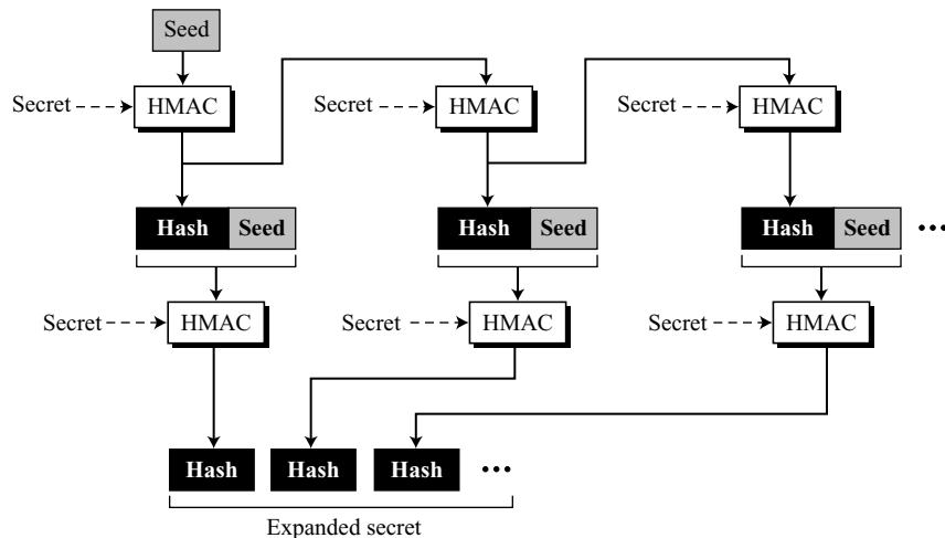
Figure 17.40 Data-expansion function
