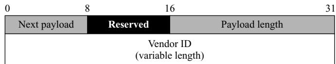
Figure 18.43 Vendor payload
