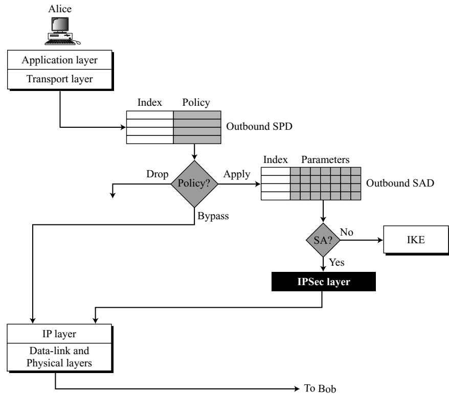
Figure 18.13 Outbound processing
