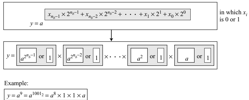
Figure 9.6 The idea behind the square-and-multiply method
