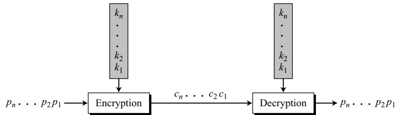
Figure 5.21 Stream cipher
