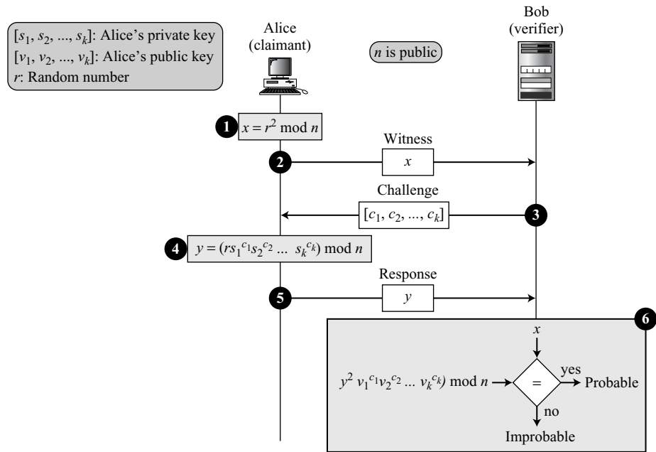
Figure 14.15 Feige-Fiat-Shamir protocol
