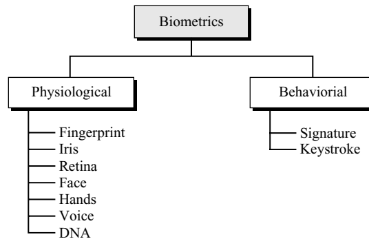
Figure 14.17 Biometrics
