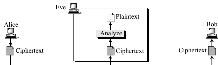
Figure 3.4 Ciphertext-only attack
