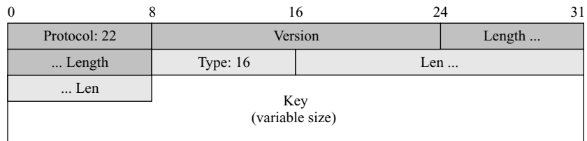
Figure 17.36 ClientKeyExchange message
