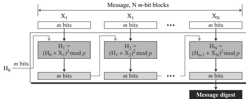
Figure 11.16 Exercise 26
