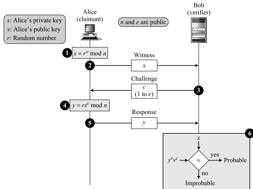
Figure 14.16 Guillou-Quisquater protocol
