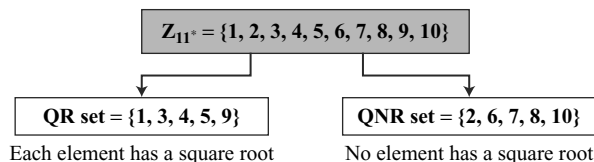
Figure 9.4 Division of \mathbf{Z}_{11}^* elements into QRs and QNRs
