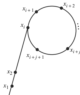
Figure 9.3 Pollard rho successive numbers
