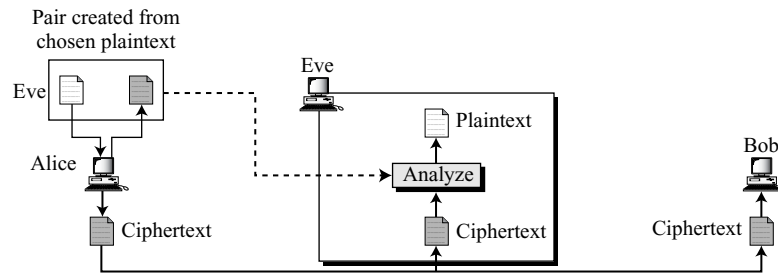
Figure 3.6 Chosen-plaintext attack
