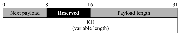
Figure 18.34 Key-exchange payload
