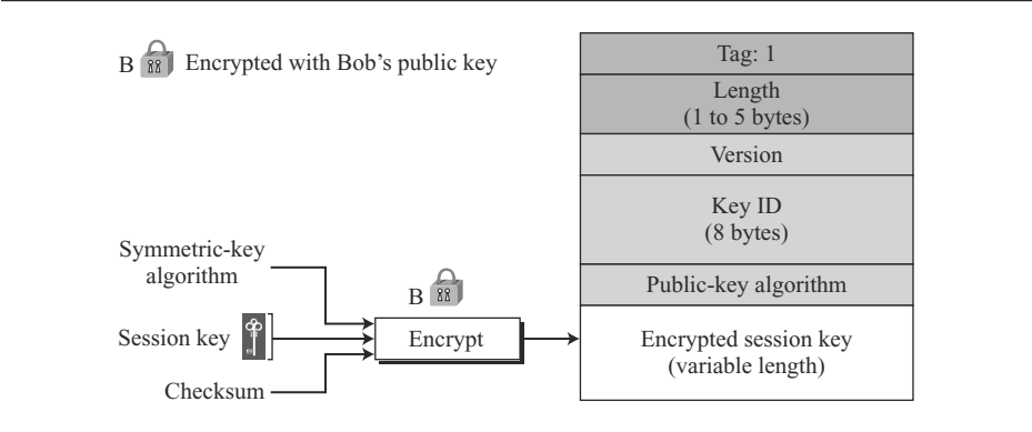
Figure 16.17 Session-key packet
