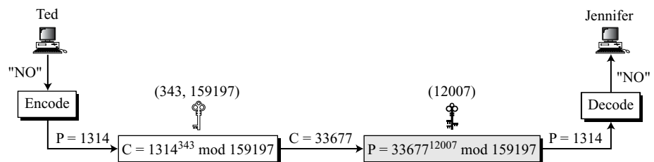
Figure 10.7 Encryption and decryption in Example 10.7
