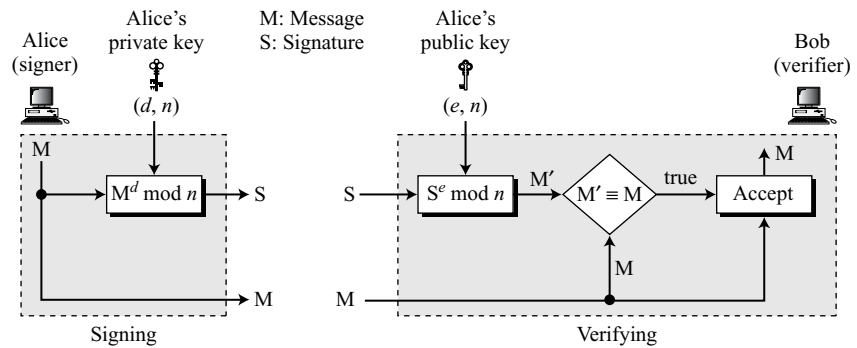
Figure 13.7 RSA digital signature scheme
