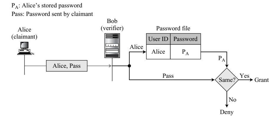
Figure 14.1 User ID and password file
