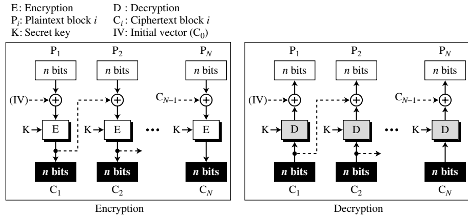
Figure 8.3 Cipher block chaining (CBC) mode
