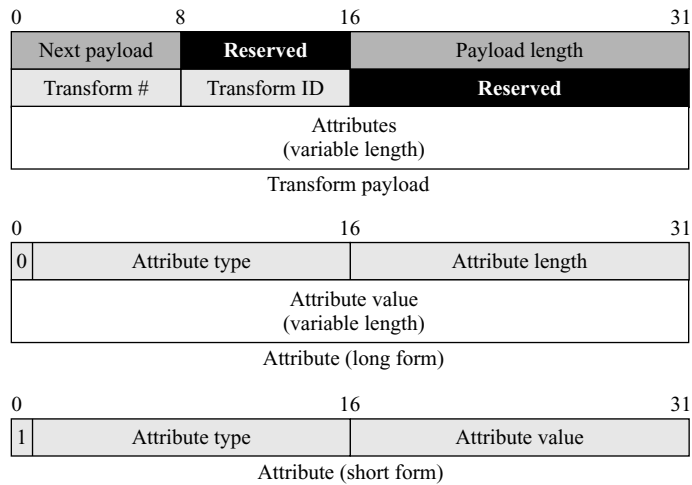
Figure 18.33 Transform payload
