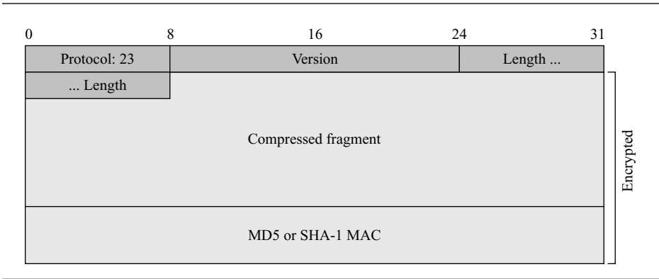
Figure 17.39 Record Protocol message for application data
