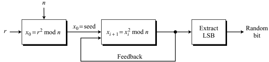
Figure K.3 Blum Blum Shub (BBC) pseudorandom number generator
