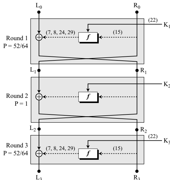
Figure N.7 A three-round characteristic for linear cryptanalysis
