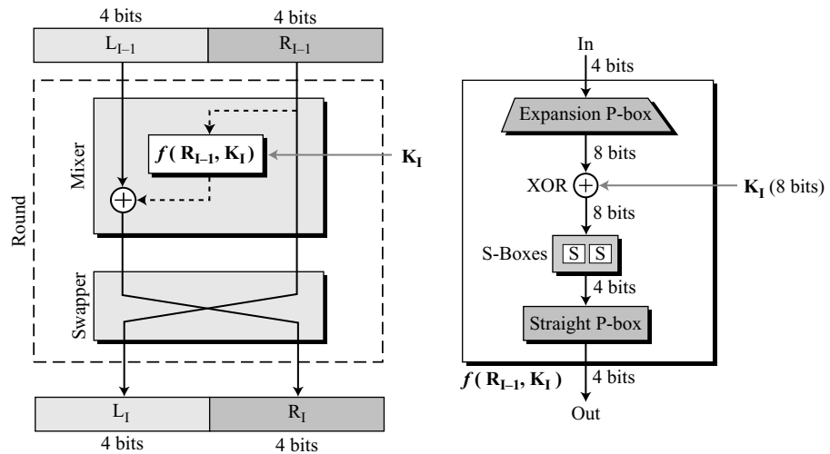
Figure O.4 A round in S-DES (encryption site)
