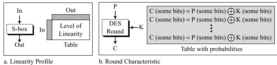
Figure N.5 Linear profile and round characteristic for DES
