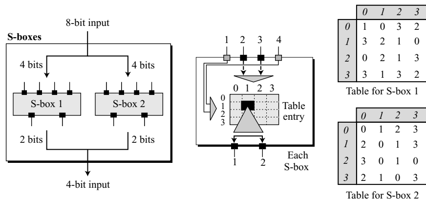
Figure O.6 S-boxes
