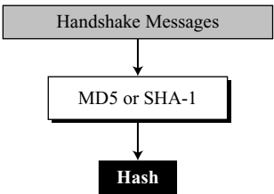
Figure 17.44 Hash for CertificateVerify message in TLS
