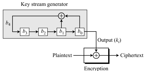
Figure 5.25 LFSR for Example 5.19
