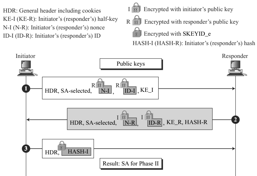
Figure 18.25 Aggressive mode, original public-key method
