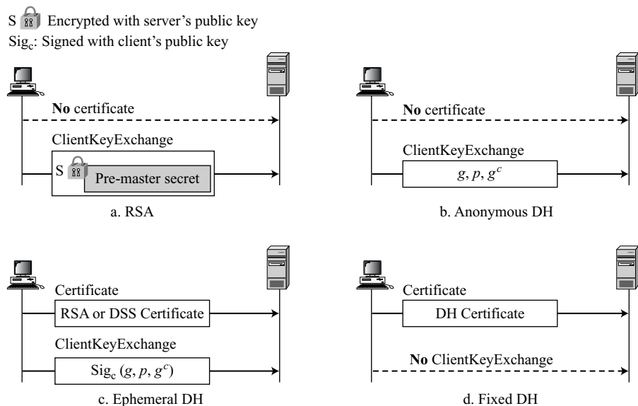
Figure 17.18 Four cases in Phase III
