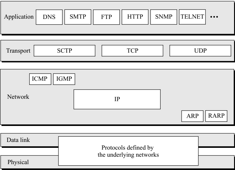
Figure C.1 TCP/IP protocol suite
