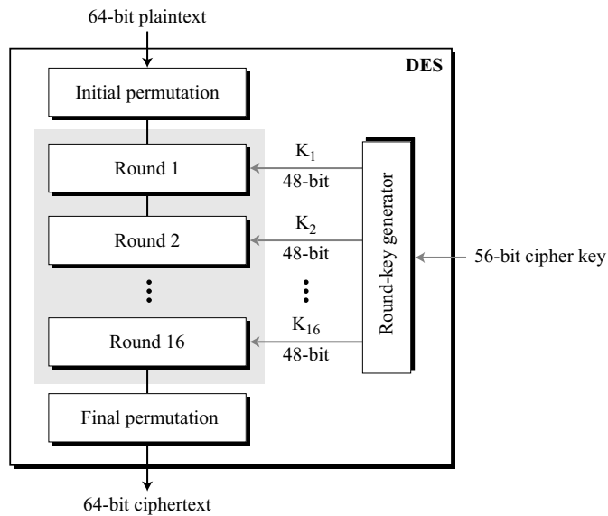
Figure 6.2 General structure of DES
