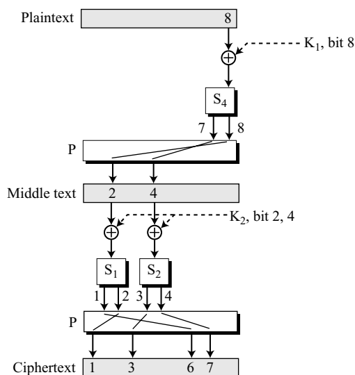
Figure 5.14 Diffusion and confusion in a block cipher
