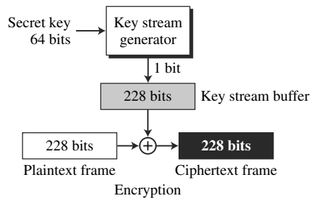
Figure 8.11 General outline of A5/1
