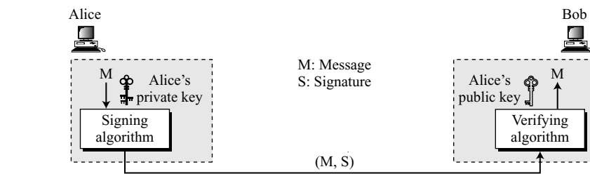
Figure 13.2 Adding key to the digital signature process
