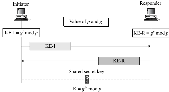
Figure 18.16 Diffie-Hellman key exchange
