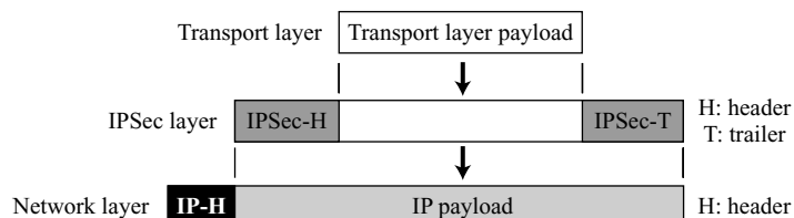
Figure 18.2 IPsec in transport mode
