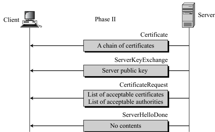
Figure 17.15 Phase II of Handshake Protocol
