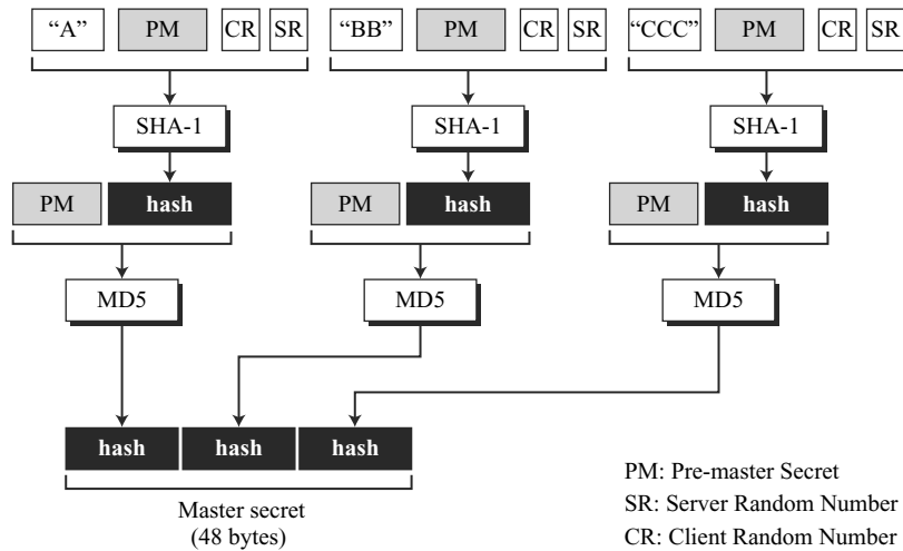
Figure 17.8 Calculation of master secret from pre-master secret
