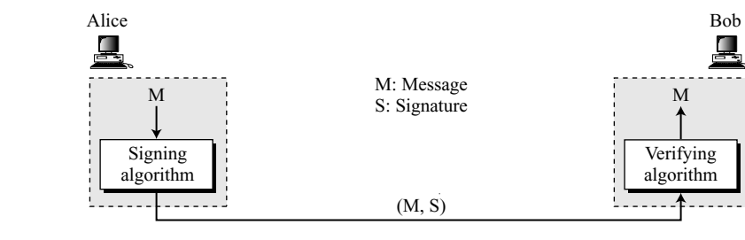
Figure 13.1 Digital signature process
