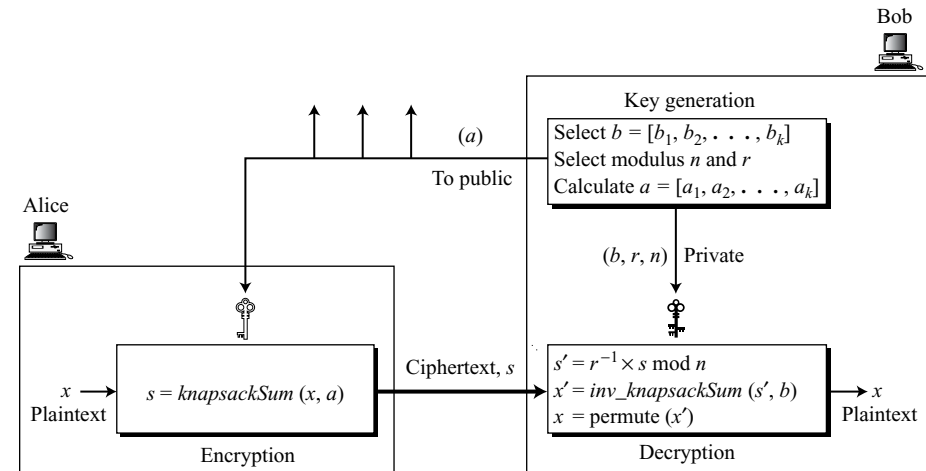
Figure 10.4 Secret communication with knapsack cryptosystem
