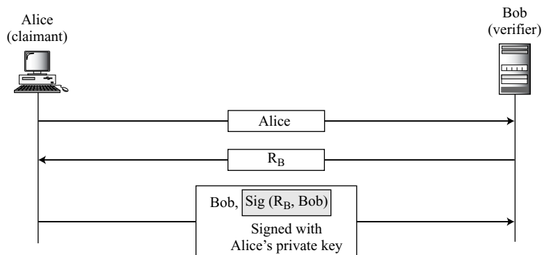
Figure 14.11 Digital signature, unidirectional authentication
