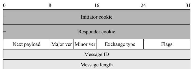
Figure 18.29 ISAKMP general header
