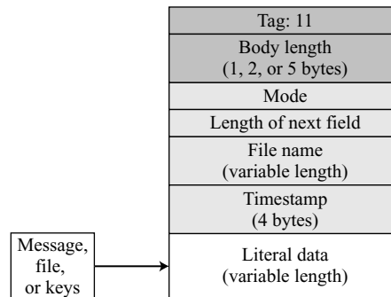
Figure 16.13 Literal data packet
