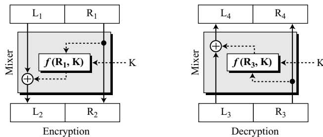
Figure 5.16 Improvement of the previous Feistel design
