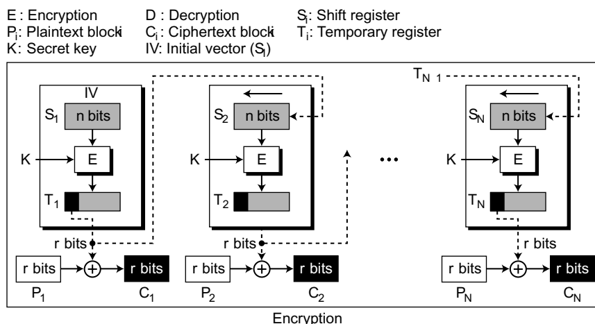
Figure 8.6 Encryption in output feedback (OFB) mode
