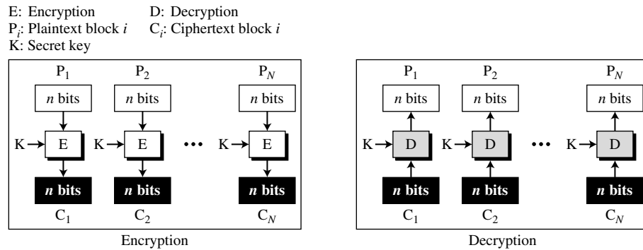
Figure 8.2 Electronic codebook (ECB) mode
