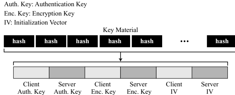
Figure 17.10 Extractions of cryptographic secrets from key material
