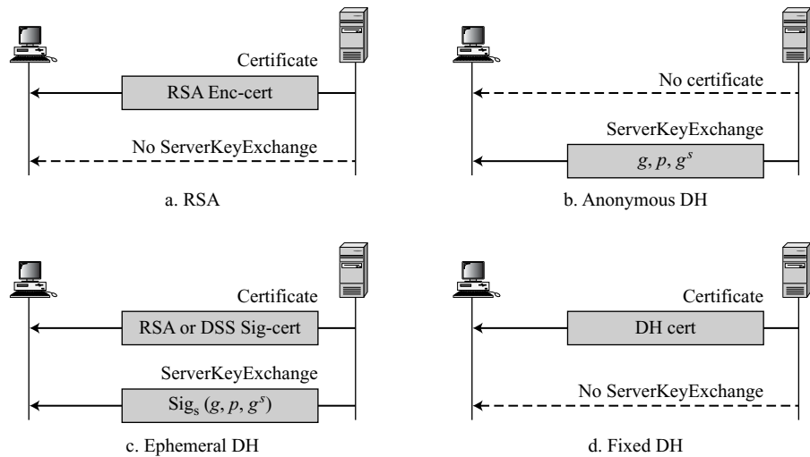
Figure 17.16 Four cases in Phase II
