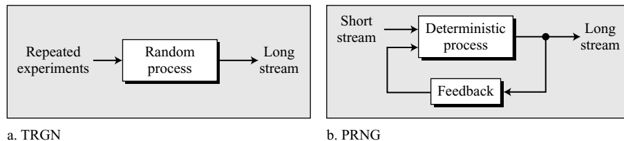
Figure K.1 TRNG and PRNG
