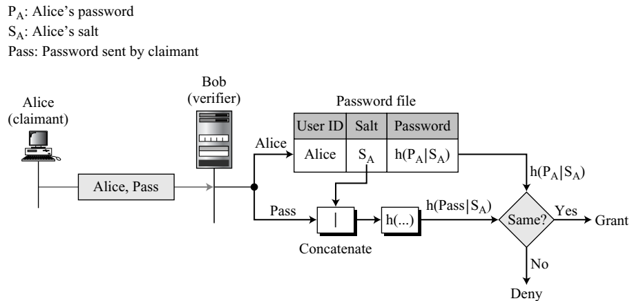
Figure 14.3 Salting the password
