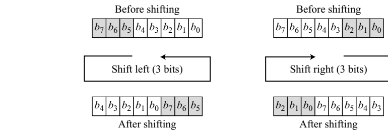
Figure 5.10 Circular shifting an 8-bit word to the left or right
