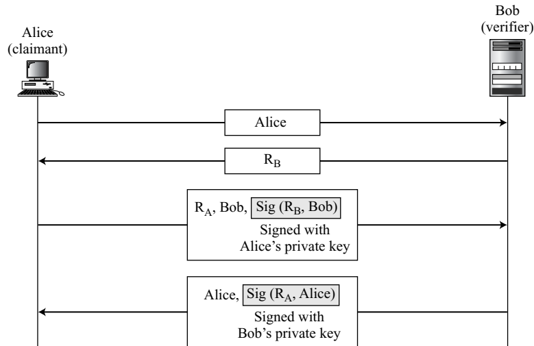
Figure 14.12 Digital signature, bidirectional authentication
