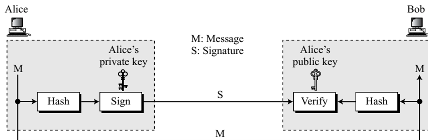
Figure 13.3 Signing the digest
