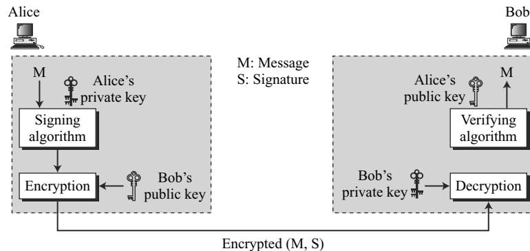
Figure 13.5 Adding confidentiality to a digital signature scheme
