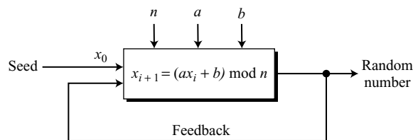
Figure K.2 Linear congruential pseudorandom number generator
