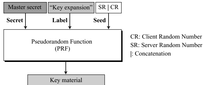
Figure 17.43 Key material generation
