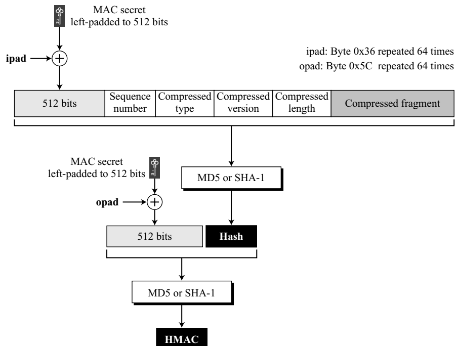
Figure 17.46 HMAC for TLS
