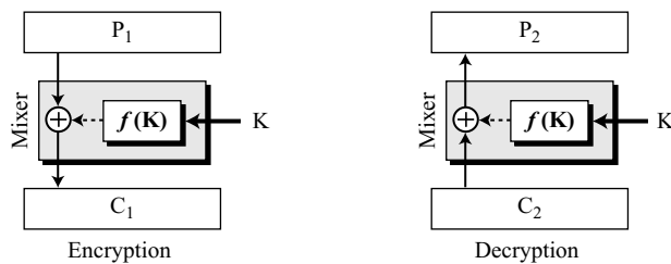
Figure 5.15 The first thought in Feistel cipher design
