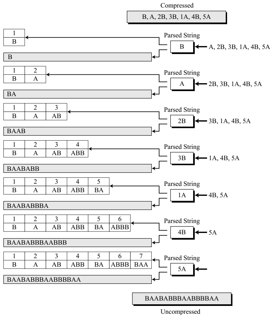
Figure M.2 Example of LZ77 decoding
