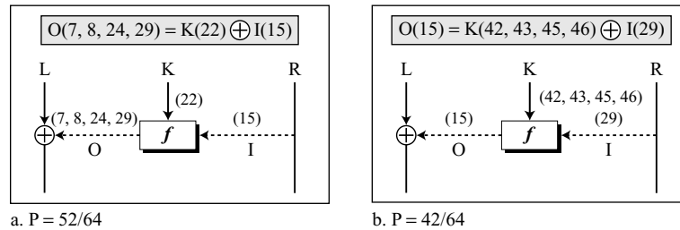
Figure N.6 Some round characteristics for linear cryptanalysis
