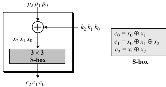
Figure 5.20 A simple cipher with a linear S-box
