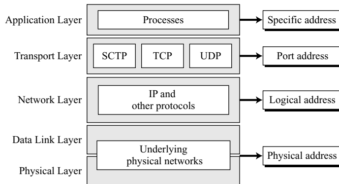
Figure C.2 Addresses in TCP/IP
