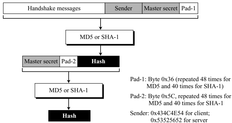
Figure 17.38 Hash calculation for Finished message
