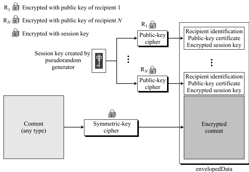
Figure 16.28 Enveloped-data content type
