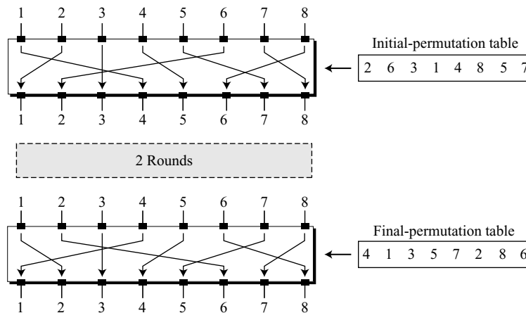
Figure O.3 Initial and final permutations ( IP and IP^{-1} )
