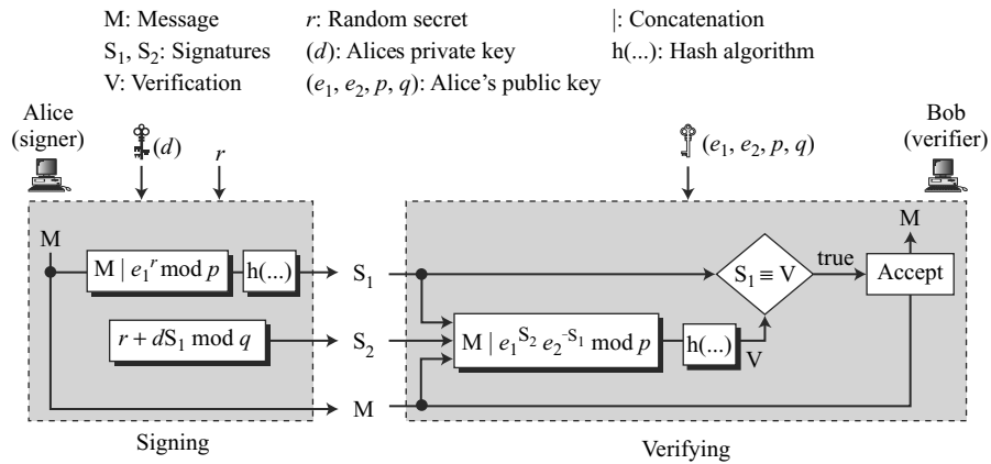
Figure 13.12 Schnorr digital signature scheme
