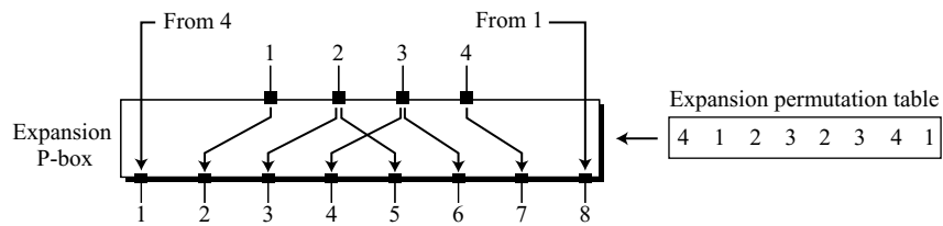
Figure O.5 Expansion P-box
