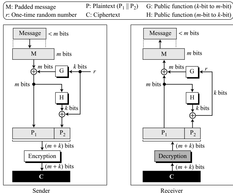
Figure 10.9 Optimal asymmetric encryption padding (OAEP)
