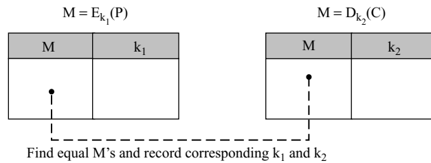
Figure 6.15 Tables for meet-in-the-middle attack
