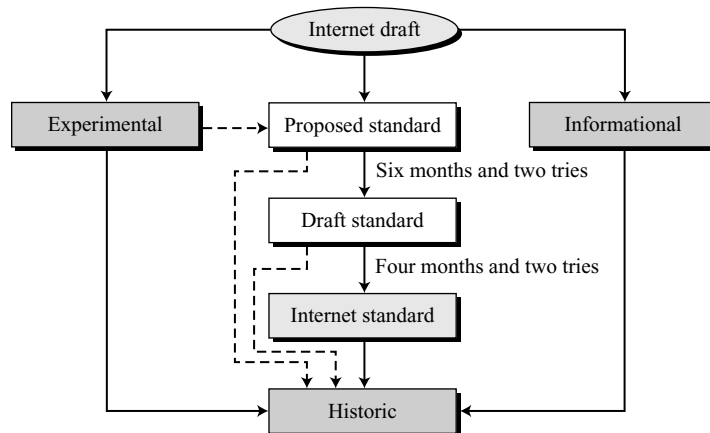
Figure B.1 Maturity levels of an RFC
