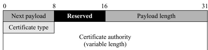
Figure 18.37 Certification request payload
