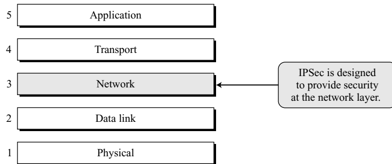
Figure 18.1 TCP/IP protocol suite and IPsec
