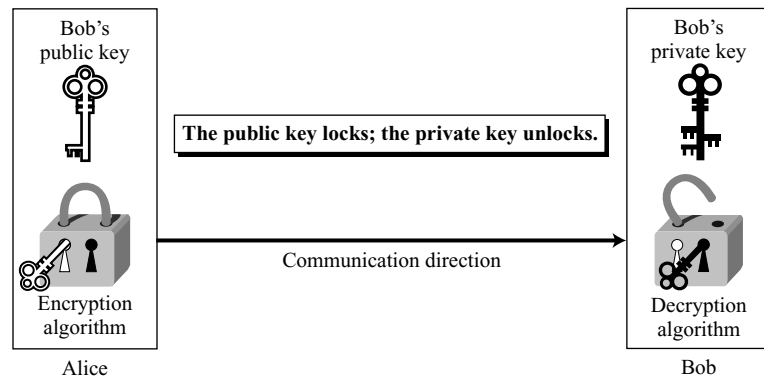
Figure 10.1 Locking and unlocking in asymmetric-key cryptosystem
