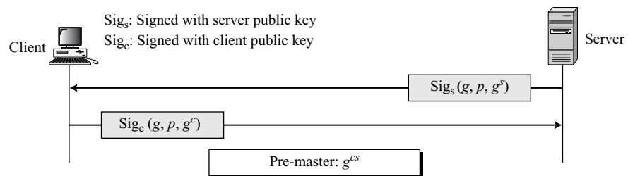
Figure 17.5 Ephemeral Diffie-Hellman key exchange
