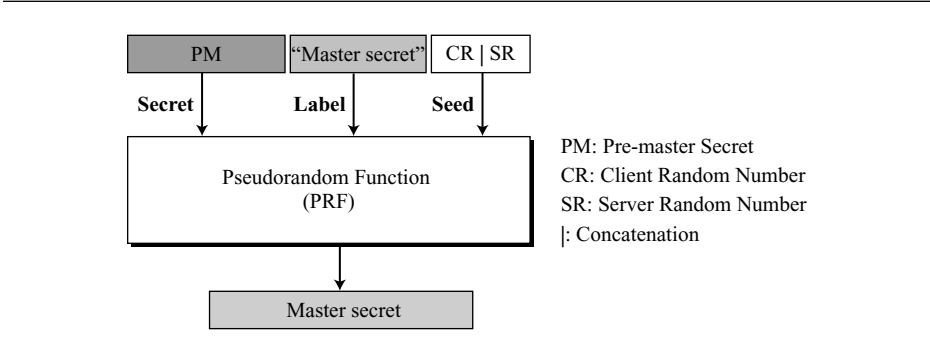
Figure 17.42 Master secret generation
