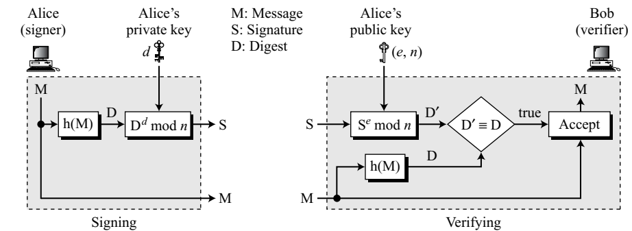
Figure 13.8 The RSA signature on the message digest
