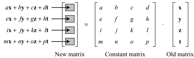
Figure 7.11 Mixing bytes using matrix multiplication
