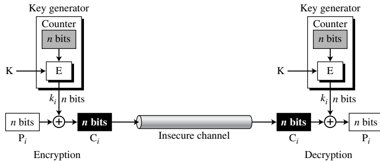
Figure 8.9 Counter (CTR) mode as a stream cipher
