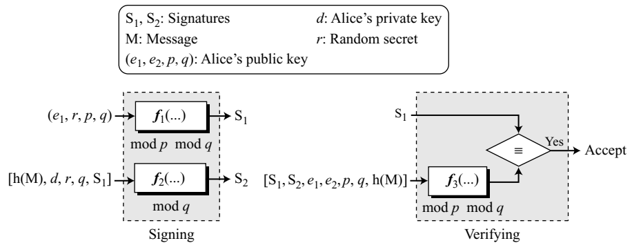
Figure 13.13 General idea behind DSS scheme
