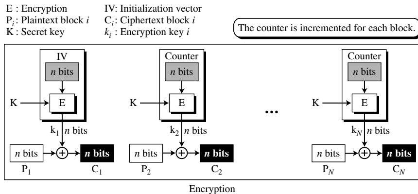
Figure 8.8 Encryption in counter (CTR) mode
