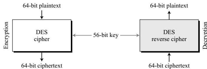
Figure 6.1 Encryption and decryption with DES
