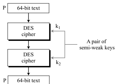
Figure 6.12 A pair of semi-weak keys in encryption and decryption
